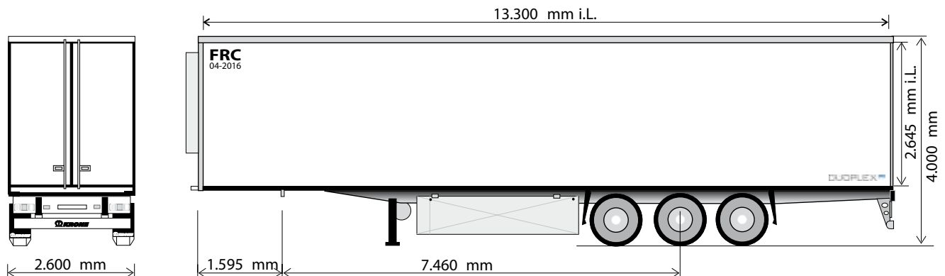
3 axle refrigerated trailer in Multitemp style with ATP/FRC certificate – side view and rear view
